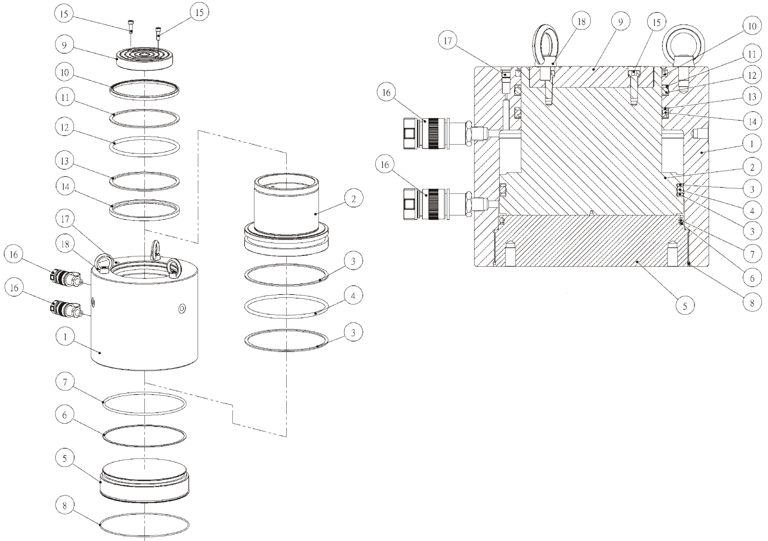
O1-Double-Acting,High Tonnage Cylinders(CSLRG-1508)
