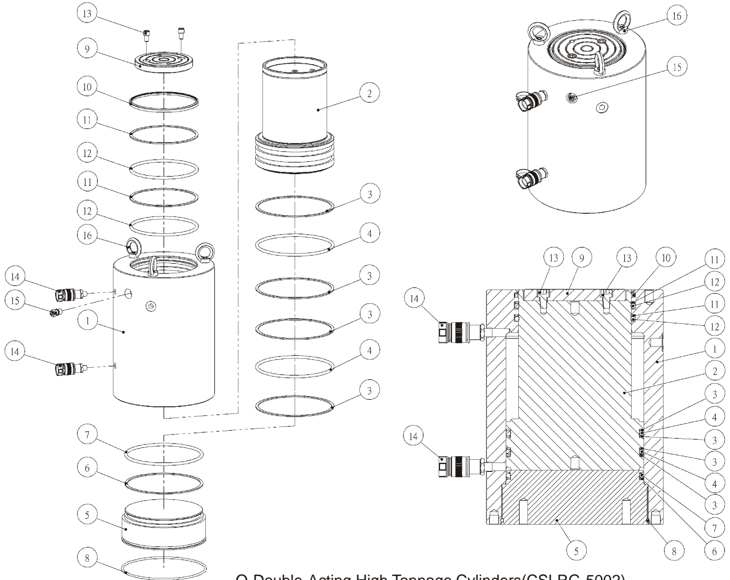
O-Double-Acting,High Tonnage Cylinders(CSLRG-5002)
