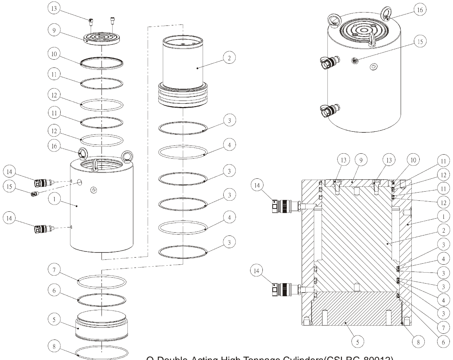
O-Double-Acting,High Tonnage Cylinders(CSLRG-80012)
