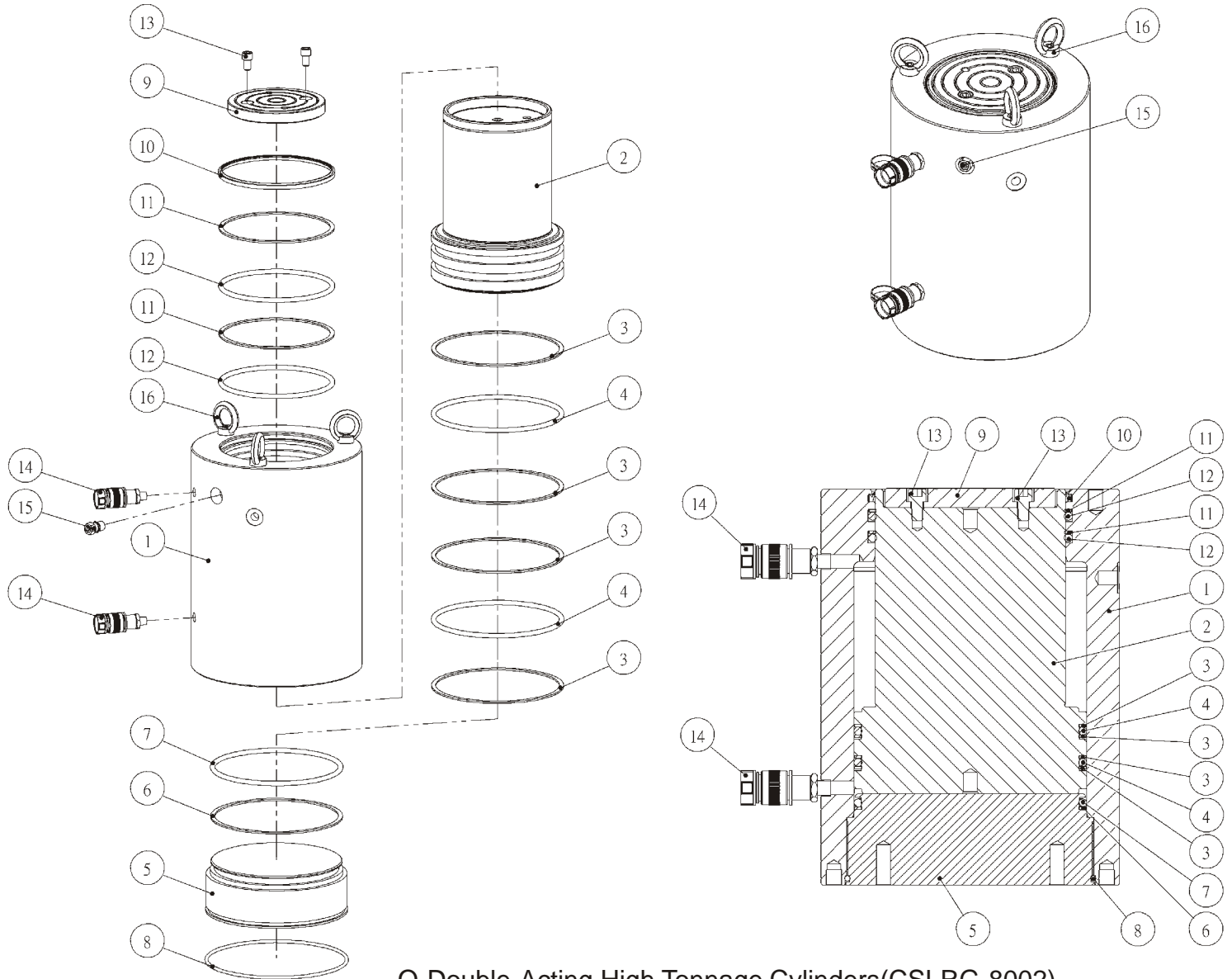
O-Double-Acting,High Tonnage Cylinders(CSLRG-8002)
