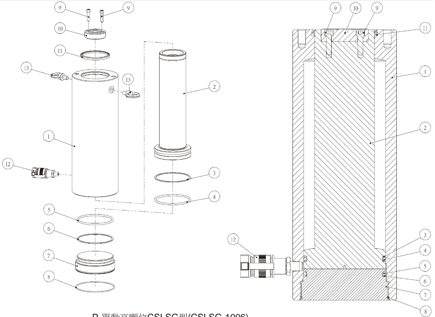
P-單動高噸位CSLSG型(CSLSG-1006)
