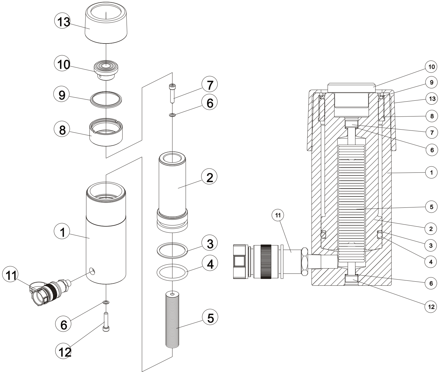
C-Single Acting, Stop ring, Plunger threads, Grooved (snap-in) saddle Cylinders (RSC-256)
