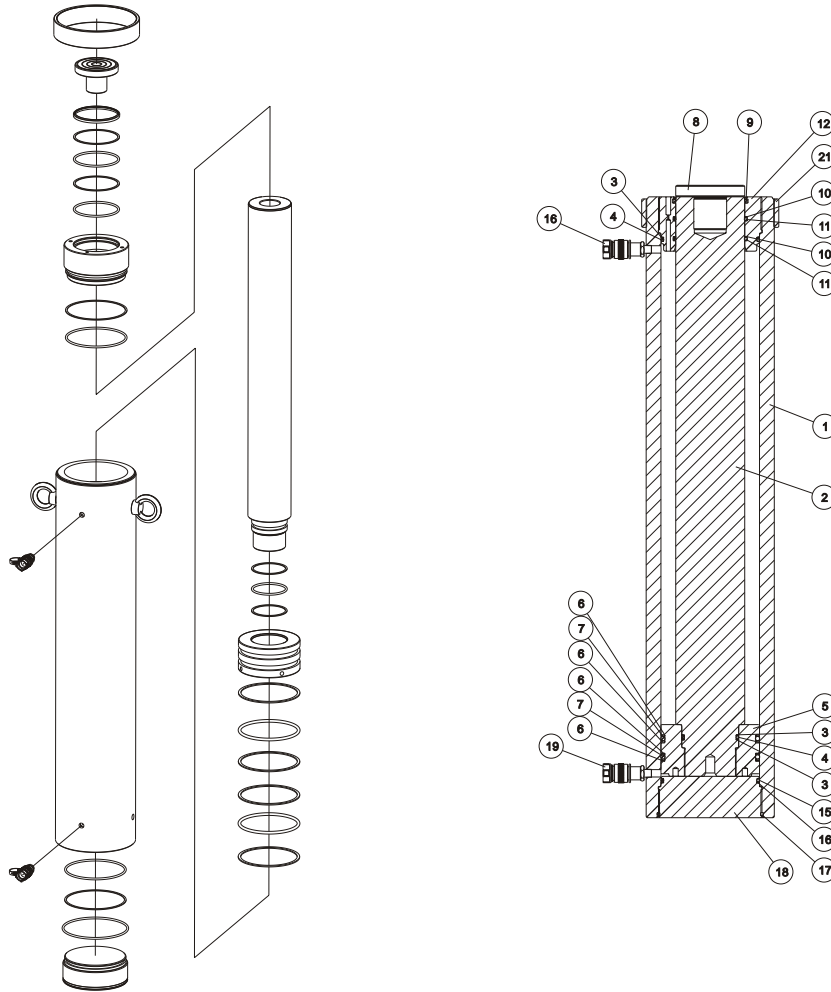
M-Double-Acting,Base,Plunger inner threads,Stop ring, Grooved saddle Cylinders(RSR-20036)
