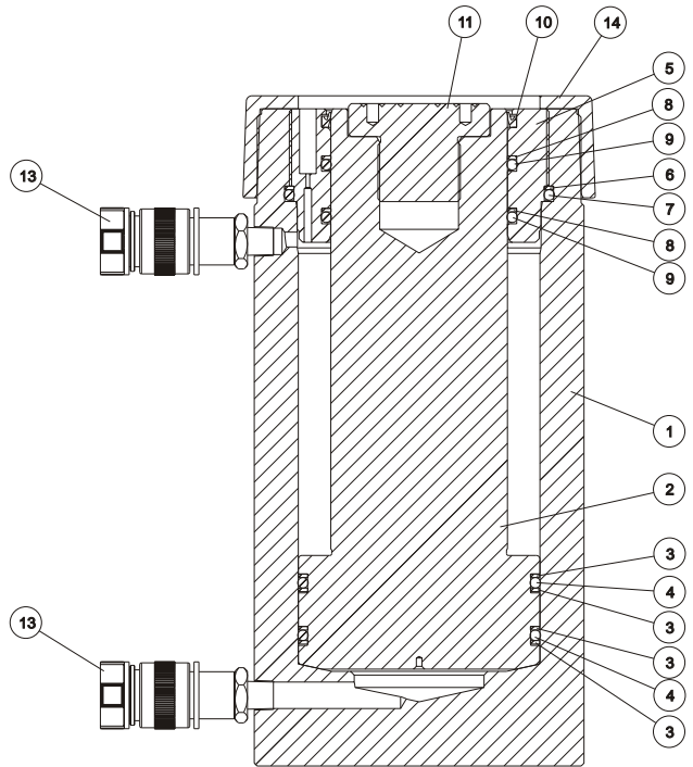
K-Double-Acting, Stop ring, Plunger threads, Safety Assembly- stop ring , Grooved saddle Cylinders (RSR-3006)
