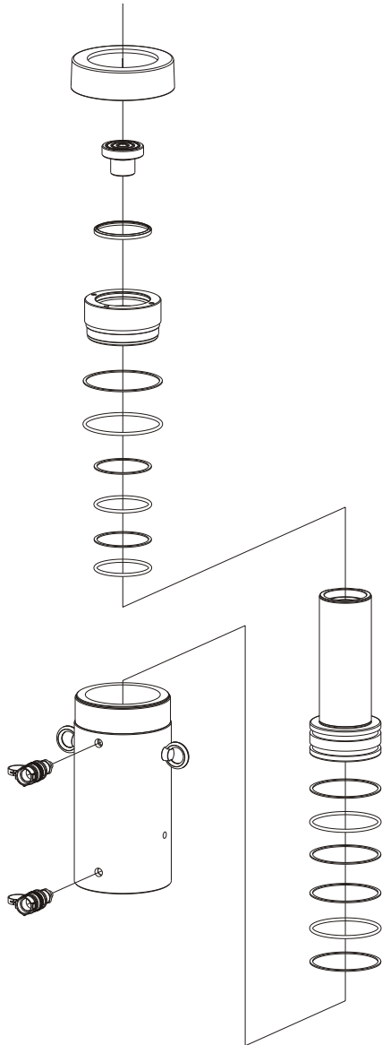
K-Double-Acting, Stop ring, Plunger threads, Safety Assembly- stop ring , Grooved saddle Cylinders (RSR-3006)
