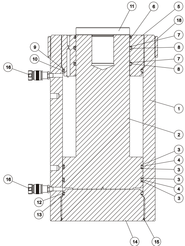
M1-Double-Acting,Base,Plunger inner thread , Stop ring,Grooved saddle Cylinders(RSR-50036)
