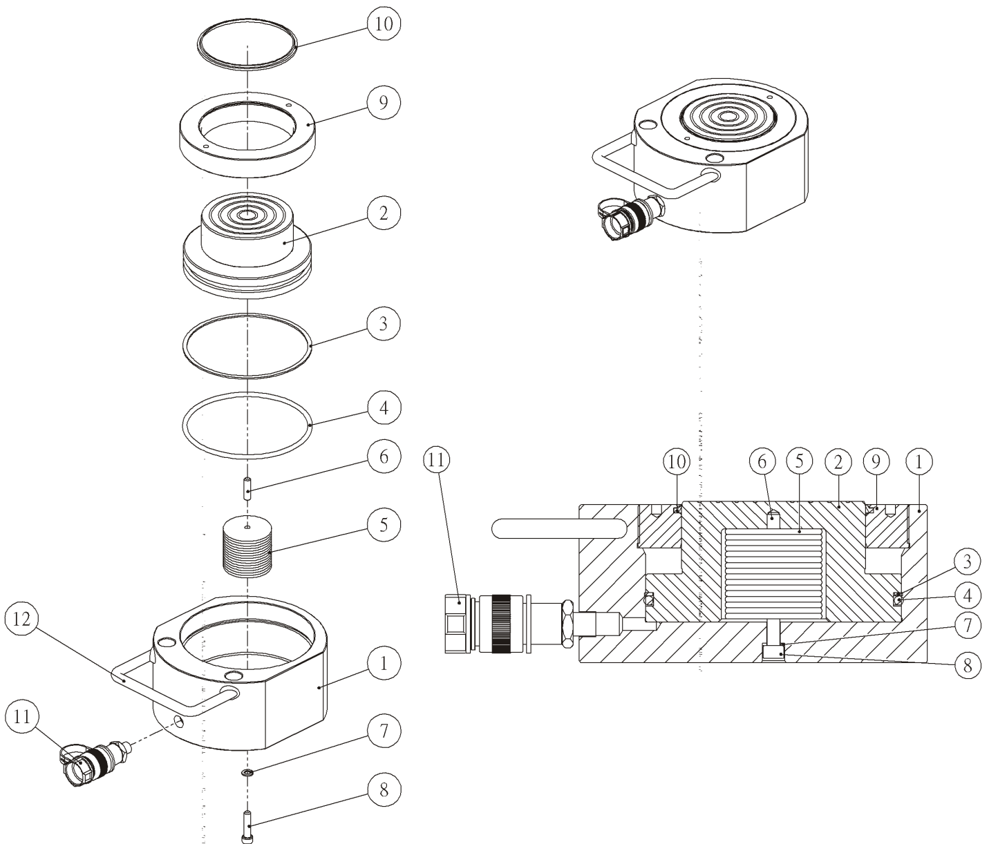
E-Single-Acting,Low Hight,Flat Cylinders (RSSM-1500)
